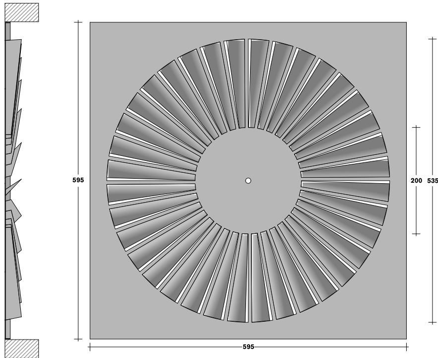
[ img.1 corte vertical [ img.2 alçado frente vue de face front view vista frontal ] coupe verticale vertical cross-section corte vertical ]
